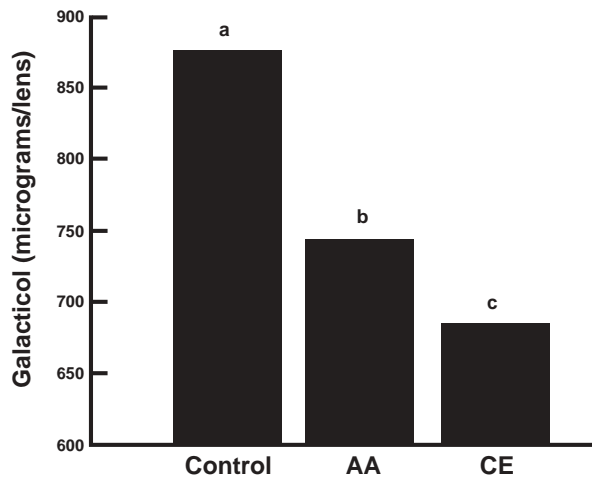
FIG. 1. Lens galacticol contents following incubation with galactose.
